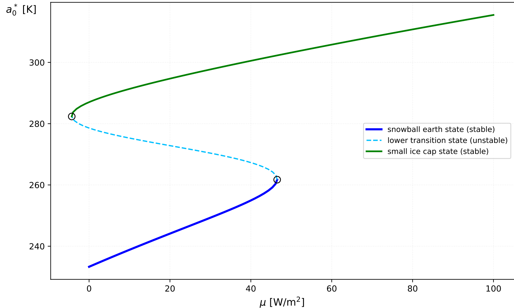
Bifurcation Diagram ( D = 30 )
